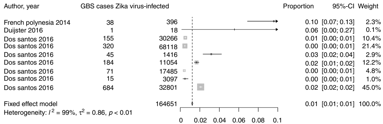
Fig. 2 – Forest plot of the prevalence of GBS associated with ZIKV infection. The plot displays pooled sample size (164,651 ZIKV-infected individuals), individual prevalence estimates by each study, pooled prevalence estimate (fixed effects model), the corresponding 95% confidence intervals, study weighting (fixed effects model) and sample size heterogeneity measures and Cochran's Q test for heterogeneity p-value.
