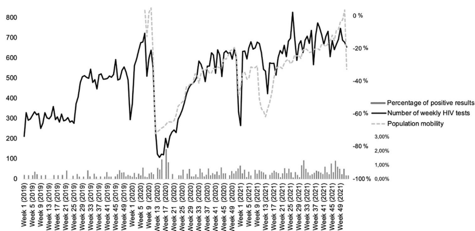
Fig. 6 – Population mobility, number of weekly tests and percentage of positive results for HIV.
