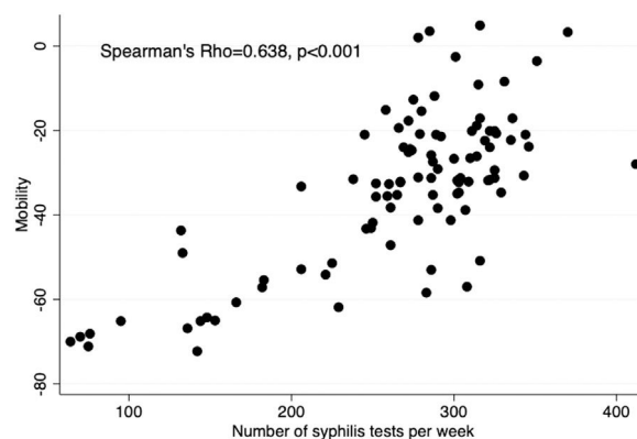
Fig. 1 – Scatter plot depicting correlations between population mobility and the number of weekly tests for syphilis.
