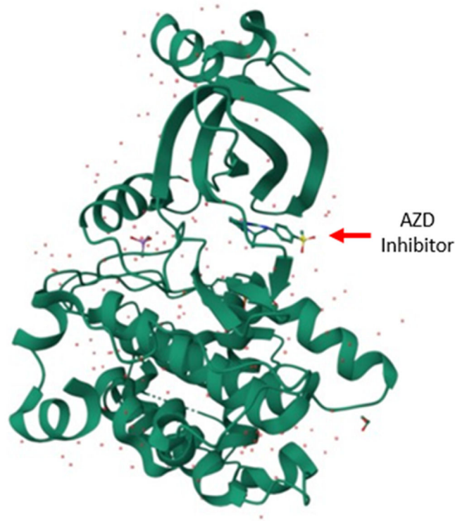
Fig. 2 – Leishmania infantum , Glycogen Synthase Kinase 3 beta bound to AZD5438 (PDB: 7S6U).
